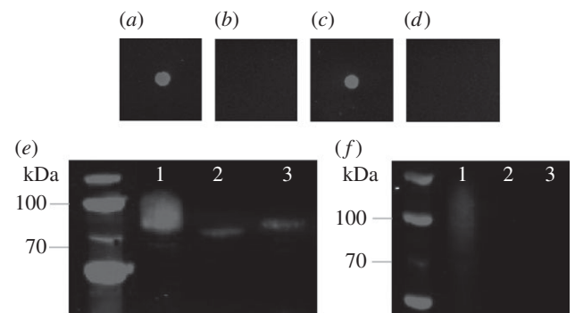
Figure 5. Glycosylation analysis of AtaC 1866–2428 alongside NGT and \alpha 6 GlcT by anti-dextran and anti-HIS western blots. Top panel: anti-dextran dot blot; (a) dextran; (b) AtaC with NGT K441A and functional \alpha 6 GlcT; (c) AtaC with functional NGT and \alpha 6 GlcT; (d) AtaC with functional NGT only. Bottom panel: anti-HIS and anti-dextran Western blots (e,f, respectively); lane 1, AtaC with functional NGT and \alpha 6 GlcT; lane 2, AtaC with NGT K441A and functional \alpha 6 GlcT; lane 3, AtaC with functional NGT only.
