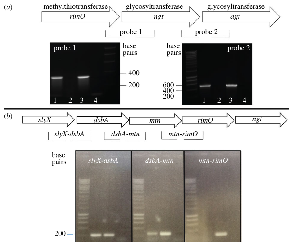
Figure 3. (a) Transcriptional analysis of the A. pleuropneumoniae NGT locus. Lane 1: cDNA as template; lane 2: RNA as template; lane 3: A. pleuropneumoniae HS143 genomic DNA positive control; lane 4: negative PCR control (no template). (b) Transcriptional analysis of the region upstream of ngt . Lane 1: cDNA as template; lane 2: genomic DNA positive control; lane 3: PCR control (RNA as template).
