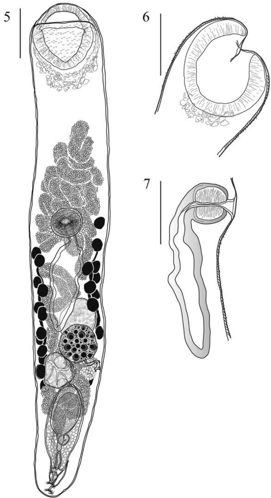
Figs. 5–7. Heterobucephalopsis perarduum n. sp. from G. javanicus from off Lizard Island. 5. Holotype, adult, whole mount, ventral view. 6. Paratype, rhynchus, lateral view. 7. Paratype, pharynx and caecum, lateral view. Scale-bars: 250 \mu m.
