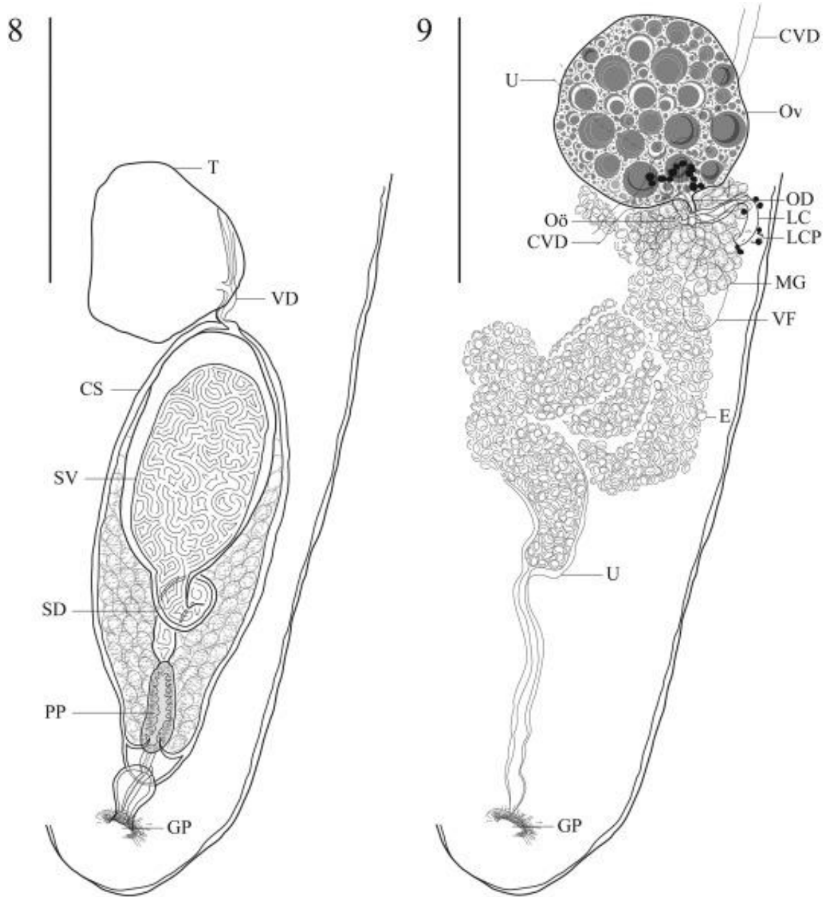
Fig. 8–9. Heterobucephalopsis perarduum n. sp. from G. javanicus from off Lizard Island. 8. Holotype, male terminal genitalia. 9. Holotype, female terminal genitalia, ventral view. Abbreviations: CS, cirrus-sac; CVD, common vitelline duct; E, egg; GP, genital pore; LC, Laurer's canal; LCP, Laurer's canal pore; MG, Mehlis' gland; OD, oviduct; Oö, oötype; Ov, ovary; PP, pars prostatica; SD, seminal duct; SV, seminal vesicle; T, testis; U, uterus; VD, vas deferens; VF, vitelline follicle. Scale-bars: 250 µm.
