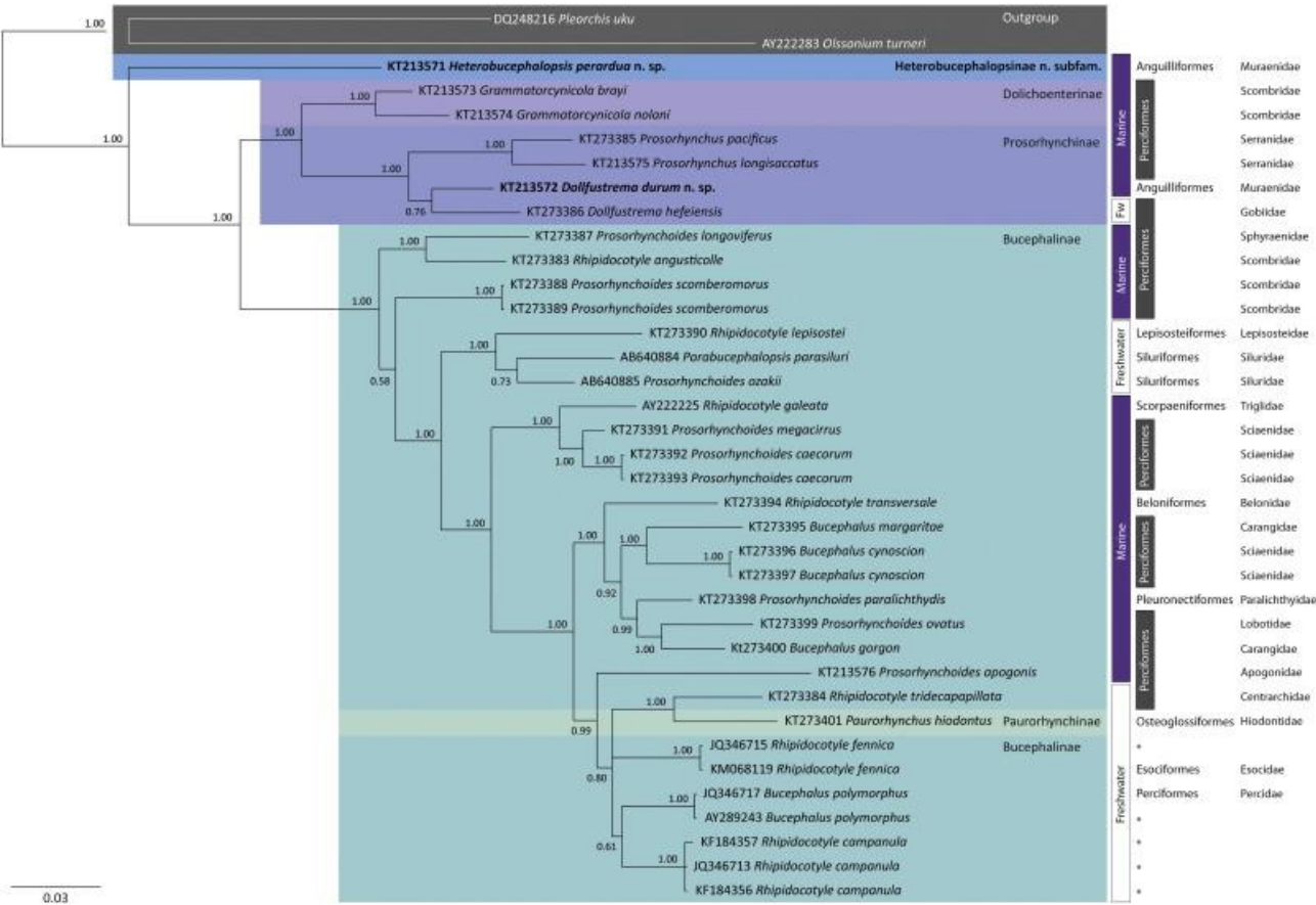
Fig. 10. The genetic relationships among species of bucephalid inferred from the D1–D3 region of the large subunit (28S) of ribosomal DNA (rDNA) locus following analysis using Bayesian inference. Posterior probabilities are indicated for all major nodes. * indicate sequence data representing bucephalid intermediate life cycle stages obtained from bivalve hosts.
