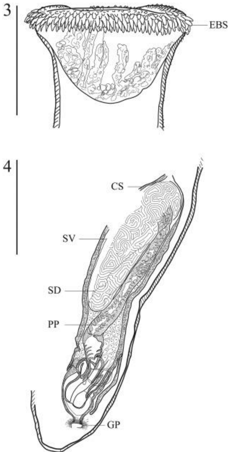
Figs. 3–4. Dollfustrema dura n. sp. from G. javanicus from off Lizard Island. 3. Holotype, rhynchus, ventral view. 4. Holotype, male terminal genitalia, ventral view. Abbreviations: CS, cirrus-sac; EBS, enlarged body spines; GP, genital pore; PP, pars prostatica; SD, seminal duct; SV, seminal vesicle. Scale bars: 200 \mu m.
