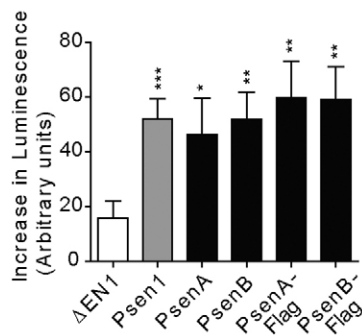
Fig. 7. The Dictyostelium presenilins are functional in mammalian cells. The PsenA and PsenB proteins were expressed in mouse-blastocyst-derived BD8 cells that have both psen1 and psen2 ablated. \gamma -secretase activity was assessed by the fold increase in luminescence resulting from cleavage of the substrate \Delta EN1 (a membrane-tethered Notch1 lacking the extracellular domain) by transfected human presenilin 1 (WT) or Dictyostelium presenilin proteins (PsenA and PsenB) with or without a C-terminal FLAG tag. Results show means \pm s.e.m. Data represent two to three independent experiments carried out in duplicate ( n=4-6 ). * P<0.05 , ** P<0.01 , *** P<0.001 .
