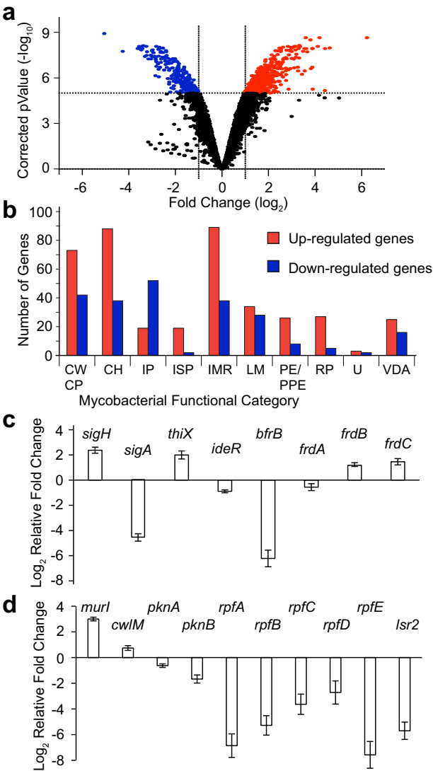
Fig. 5 | Mtb exposure to NOD for 4 h led to activation of several regulatory pathways. a Volcano plot showing 407 genes significantly induced (red) and 233 genes repressed (blue) by NOD compared to CC at 4 h. Significantly differentially expressed genes (DEG) were identified using a moderated t -test ( p < 5 \times 10^{-5} with Benjamini and Hochberg multiple testing correction) and fold change > 2.0 . b Distribution of DEG from functional categories 69 . CWCP cell wall and cell processes, CH conserved hypothetical, IP information pathways, ISP insertion sequences and phages, IMR intermediary metabolism and respiration, LM lipid metabolism, RP regulatory proteins, U unknown, VDA virulence, detoxification, adaptation. c , d Expression of selected genes was confirmed by RT-qPCR, normalized to 16S rRNA transcript abundance. \log_2 relative fold difference was calculated. Data are means \pm SEM for three independent cultures done in technical duplicates ( n = 6 ).
