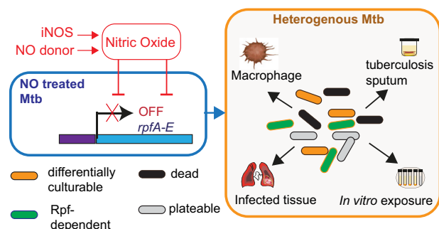
Fig. 7 | NO-mediated generation of Rpf-dependent DC Mtb. NO exposure in vivo and in vitro shuts down expression of rpfA , rpfB , rpfC , rpfD and rpfE . This leads to generation of heterogeneous Mtb subpopulations including Rpf-dependent Mtb. This population heterogeneity mimics in vivo observations where NO is produced by the inducible NO synthase (iNOS) and drives formation of Rpf-dependent and differentially culturable Mtb that can be detected in infected tissue and sputum samples.
