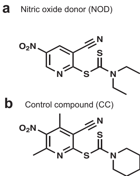
Fig. 2 | Chemical structures of the nitric oxide donor (NOD) and control compound (CC). a NOD 3-cyano-5-nitropyridin-2-yl diethyldithiocarbamate and b CC 6-dimethyl-5-nitropyridin-2-yl piperidine-1-carbodithioate.
